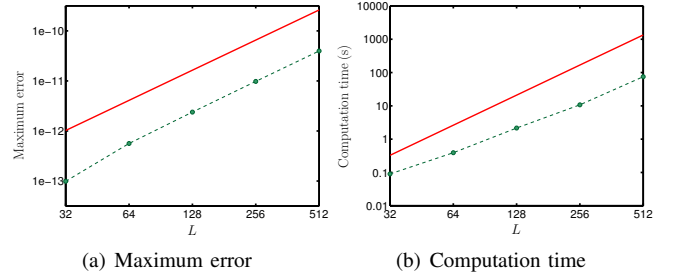
Fig. 2. Numerical accuracy and computation time of the spherical ridgelet transform, averaged over ten round-trip transforms of random test signals. Numerical accuracy close to machine precision is achieved and found empirically to scale as \mathcal{O}(L^2) , with a factor of \mathcal{O}(L) coming from the inversion of each of the spherical Radon and spherical wavelet transforms. Computation time is found empirically to scale as \mathcal{O}(L^3) , as expected theoretically. \mathcal{O}(L^2) and \mathcal{O}(L^3) scaling is shown by the solid red lines in panels (a) and (b) respectively.
